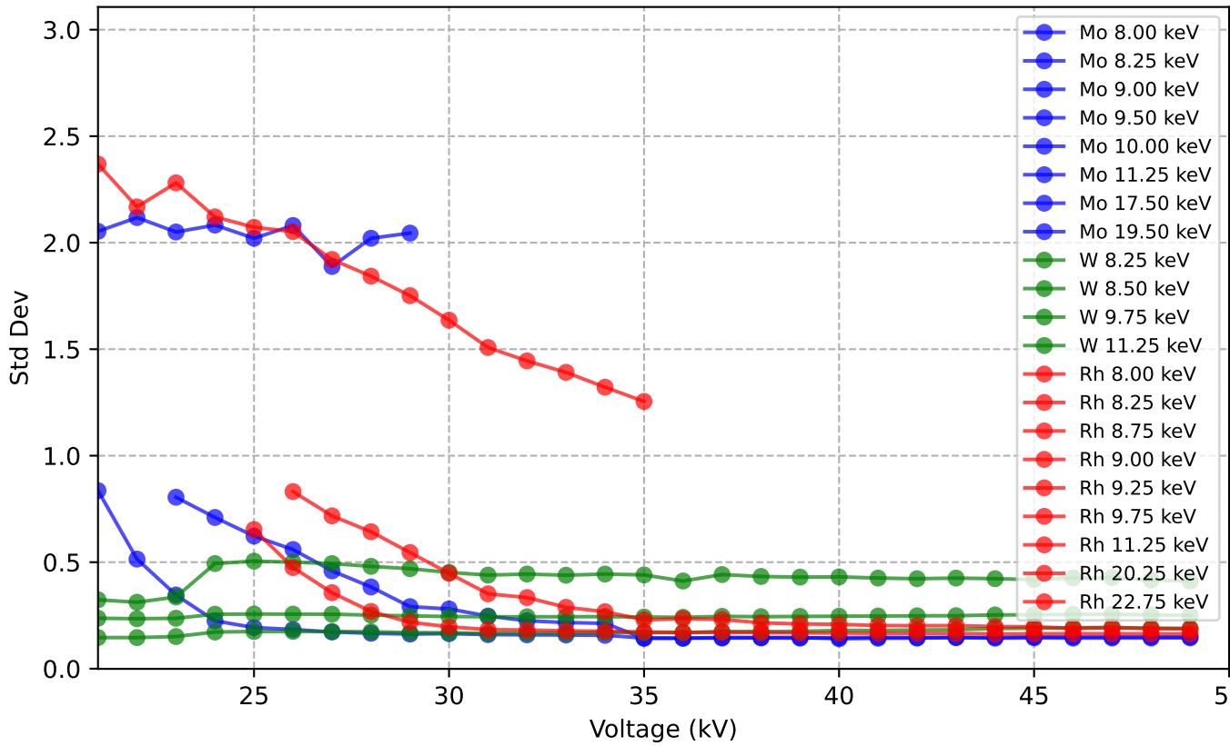
Std Dev vs Voltage
